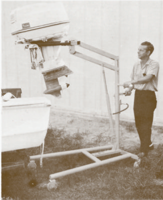
BUILT TO RAISE HIGH TO SOLVE MOTOR STORAGE PROBLEMS
